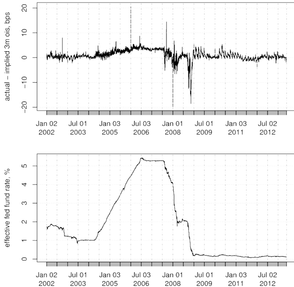
Figure 8: Calibration result, for period between 2002-01-02 and 2013-05-29, \lambda = 0.0 . Top panel: difference between the actual and the implied 3-month OIS fixings, in basis points. Bottom panel: time series of the effective fed fund rate over the sample period.
