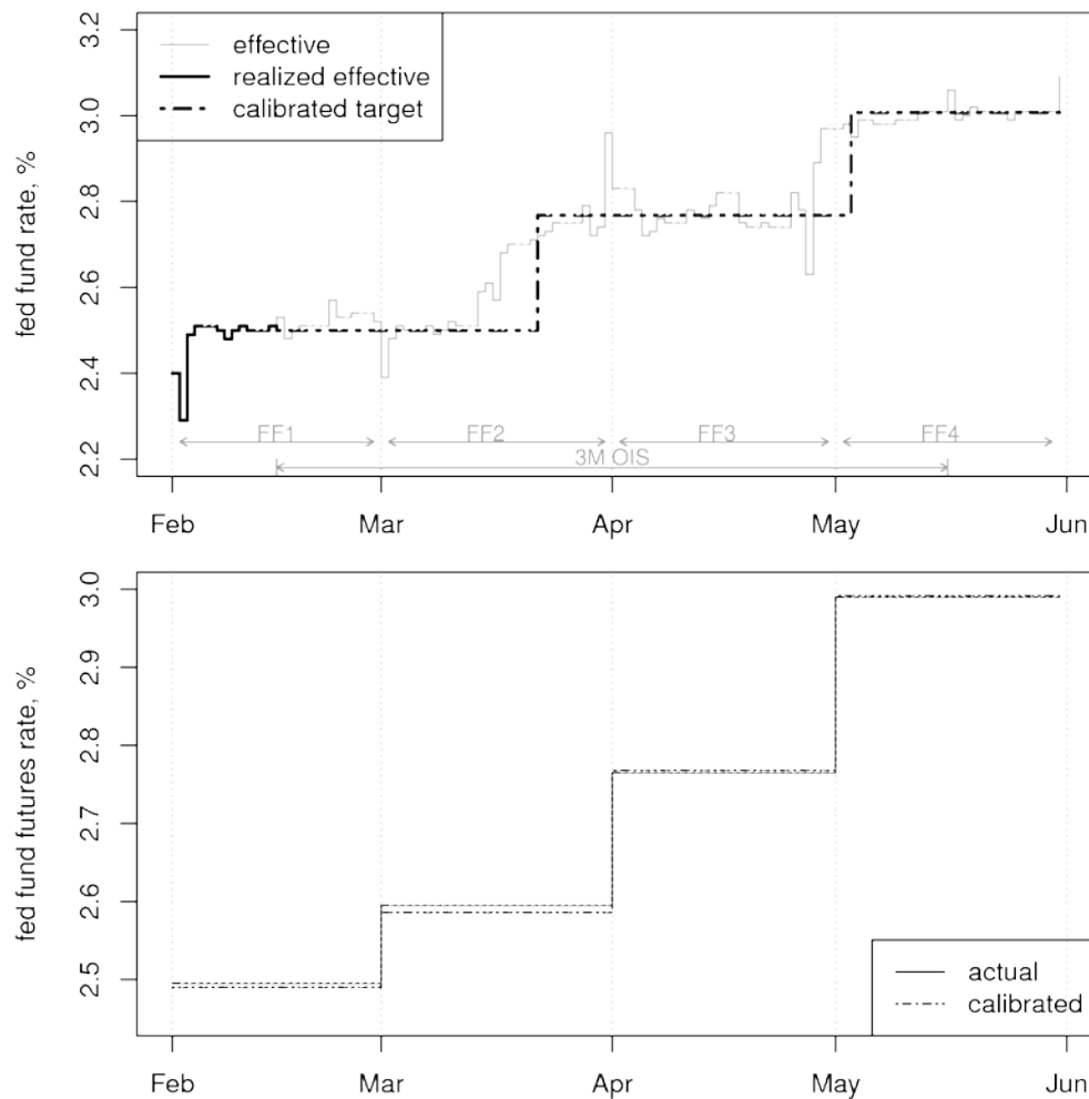
Figure 7: An example that illustrates the various components of the calibration process, together with the result, for a 3-month OIS term contract, with settlement date on 2005-02-15 and termination date on 2005-05-15, \lambda = 0.0 . The labels FF1 to FF4 indicate the span of the front, second, third and fourth fed fund futures contract. The label 3M OIS indicates the span of the 3-month OIS term contract. Top panel: solid black line is the realized effective fed fund rate between 2005-02-01 and 2005-02-15; dash-line is the expected target fed fund rate; gray solid line is the historical effective fed fund rate. Bottom panel: solid black line is the actual market fed fund rate based on the closing price on 2005-02-11; dash-line is the implied rate based on the calibration procedure outlined in this section.
