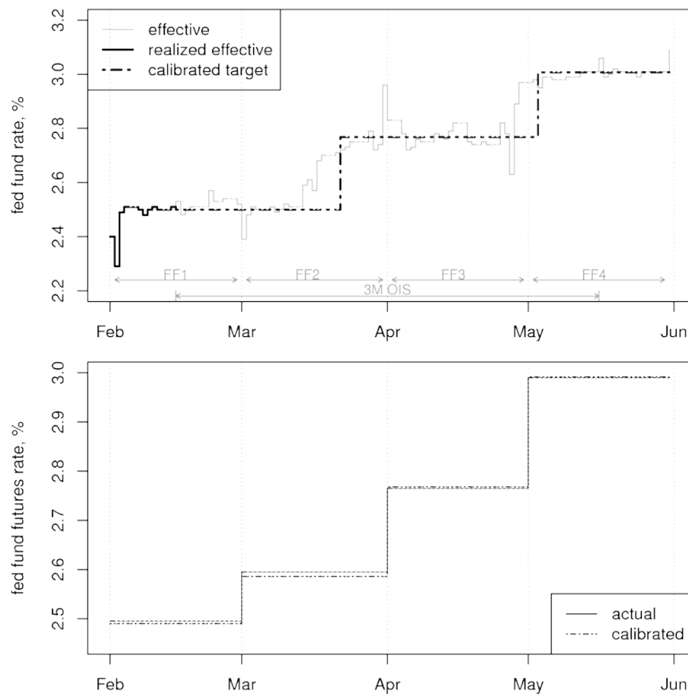
Figure 3: An example that illustrates the various components of the calibration process, together with the result, for a 3-month OIS term contract, with settlement date on 2005-02-15 and termination date on 2005-05-15, \lambda = 0.0 . The labels FF1 to FF4 indicate the span of the front, second, third and fourth fed fund futures contract. The label 3M OIS indicates the span of the 3-month OIS term contract. Top panel: solid black line is the realized effective fed fund rate between 2005-02-01 and 2005-02-15; dash-line is the expected target fed fund rate; gray solid line is the historical effective fed fund rate. Bottom panel: solid black line is the actual market fed fund rate based on the closing price on 2005-02-11; dash-line is the implied rate based on the calibration procedure outlined in this section.
