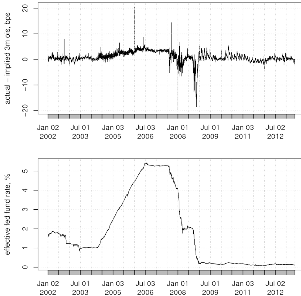
Figure 4: Calibration result, for period between 2002-01-02 and 2013-05-29, \lambda = 0.0 . Top panel: difference between the actual and the implied 3-month OIS fixings, in basis points. Bottom panel: time series of the effective fed fund rate over the sample period.
